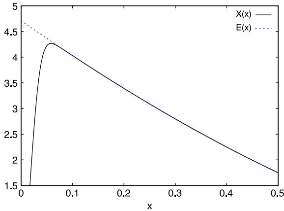
Fig. 11. Extrapolation of X_{500}(x) for the ellipse.
